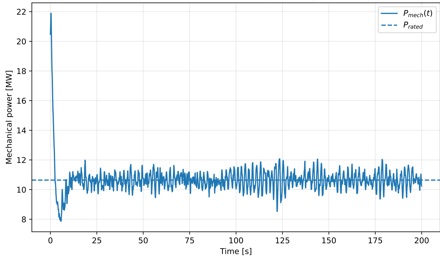
Turbulent wind: mechanical power response
